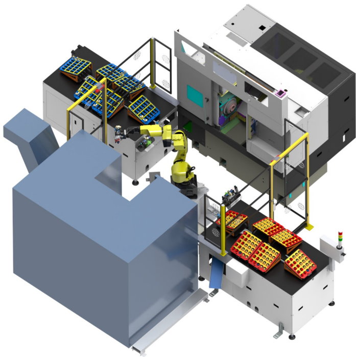
客製夾爪組 Customized gripper
